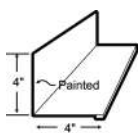
LG 109 DENVER SIDEWALL FLASHING
