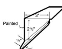
LG 131 NATIONAL DOOR TRACK COVER
