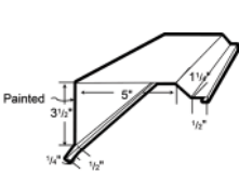
LG 129 WINDOW DRIP CAP*
